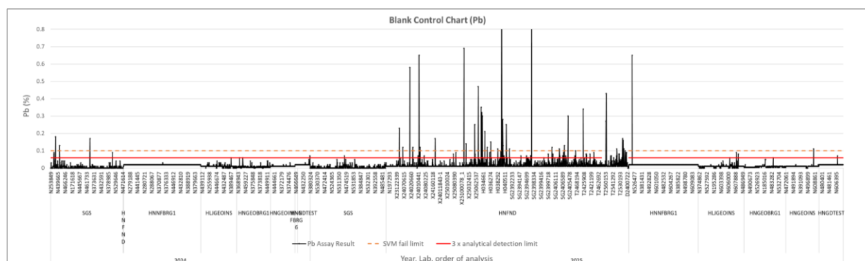
Figure 11.12 Coarse blank control chart (Pb)
