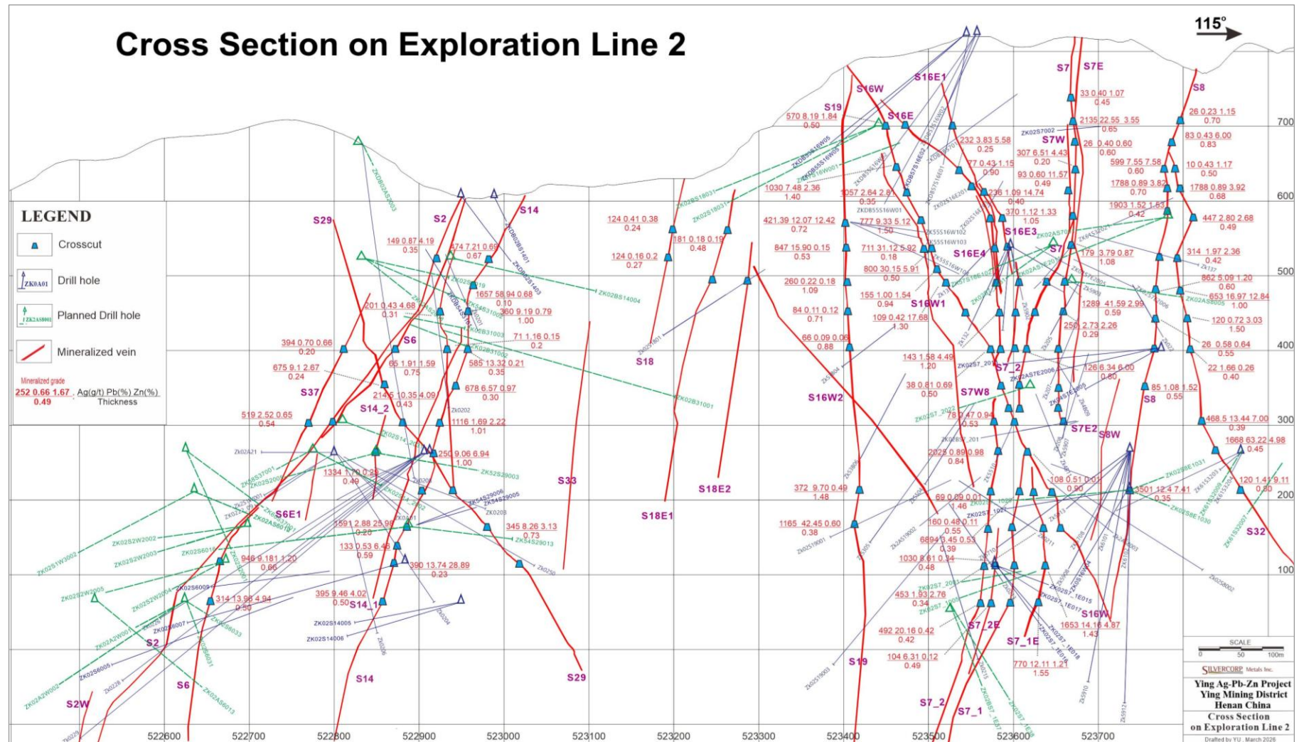
Figure 7.5 Cross section on Line 2, SGX
