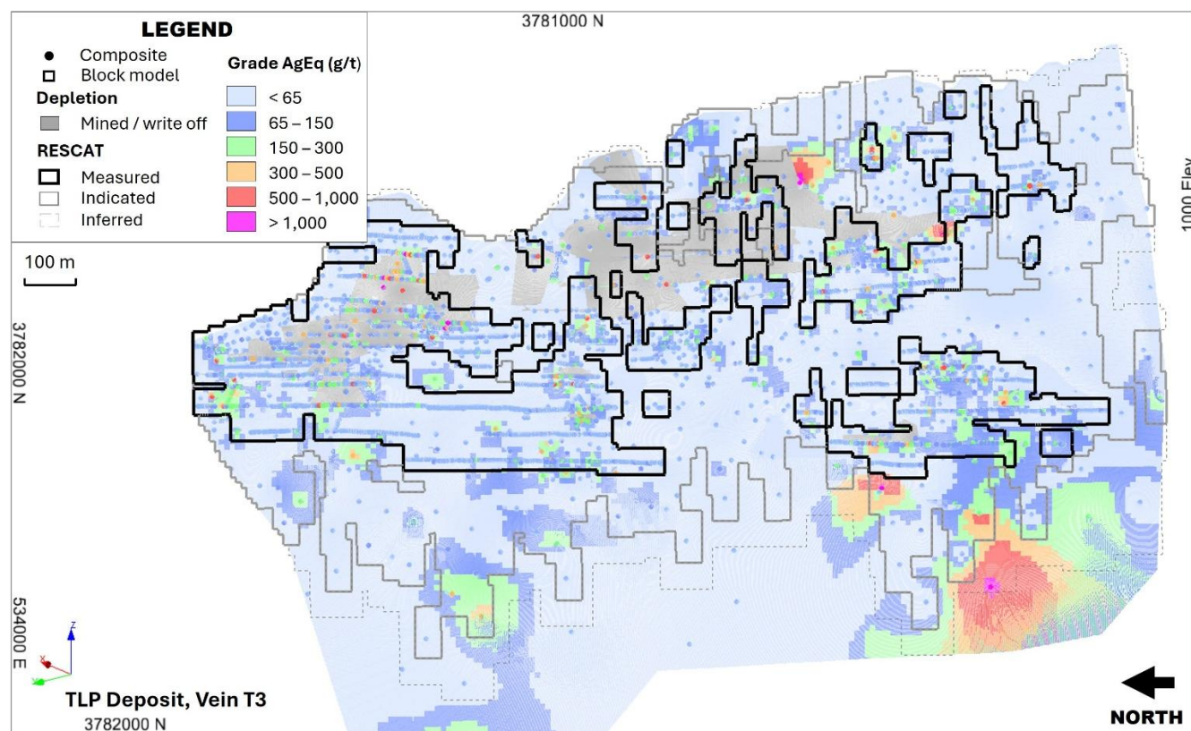
Figure 14.26 TLP - Vein T3 vertical long section projection Mineral Resource
