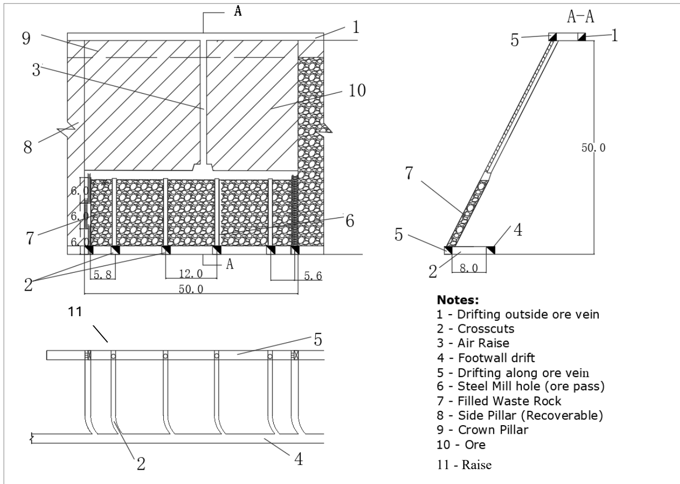
Figure 16.8 Resue stoping method
