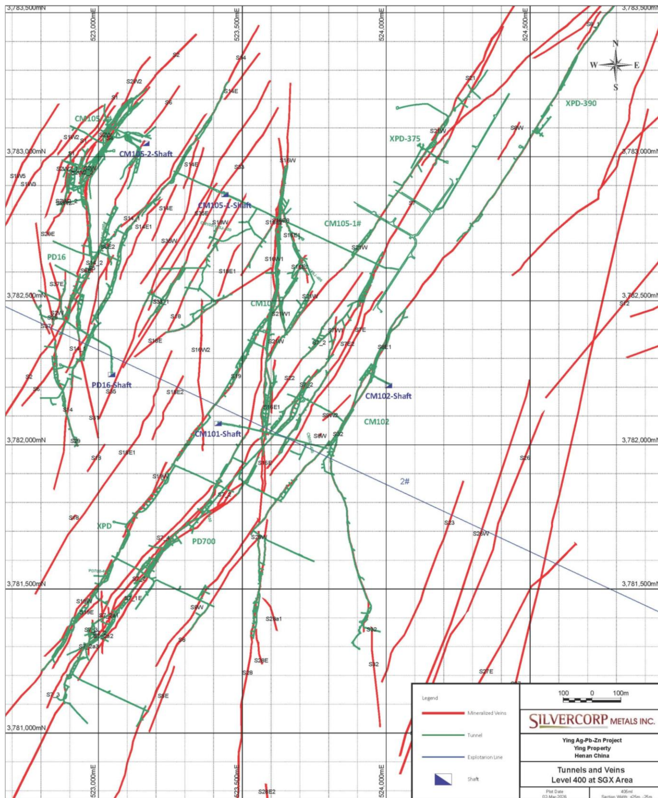
Figure 7.4 Tunnels and veins in the SGX area
