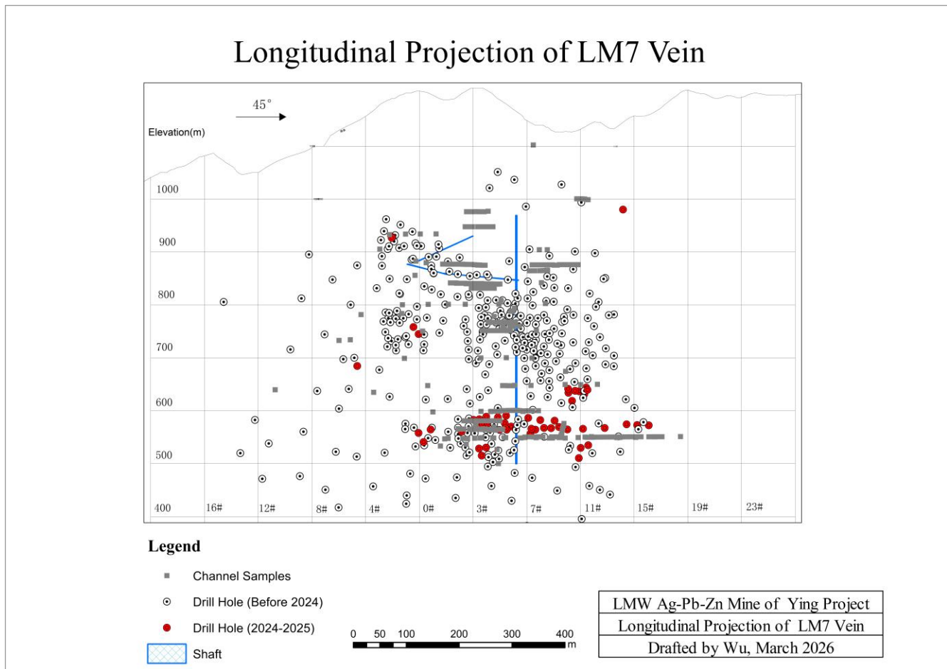
Figure 9.6 Longitudinal projection of Vein LM7, LMW
