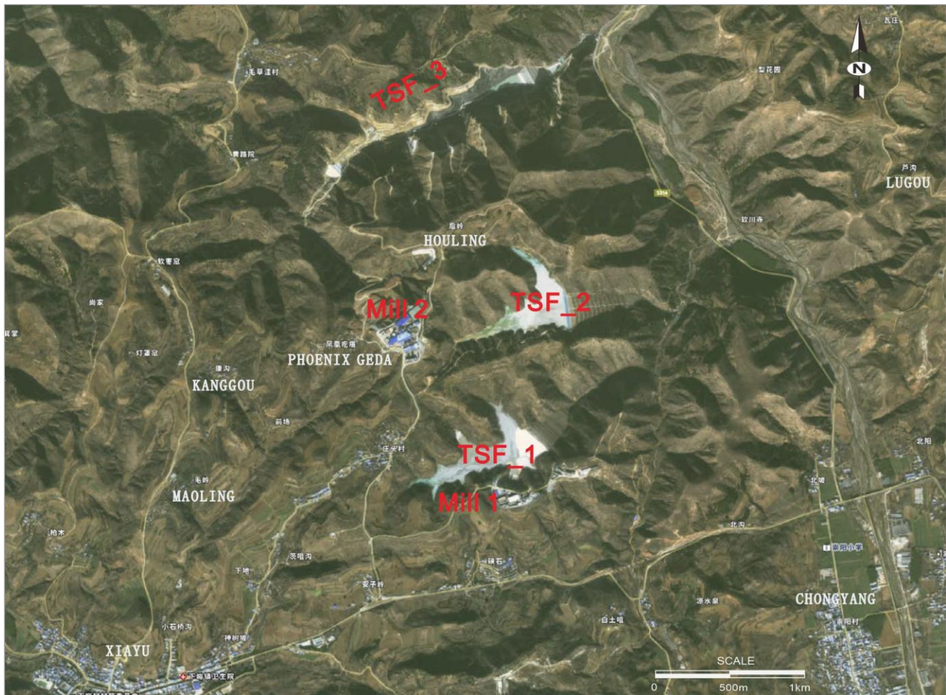
Figure 18.1 Arrangement of Ying TSFs
