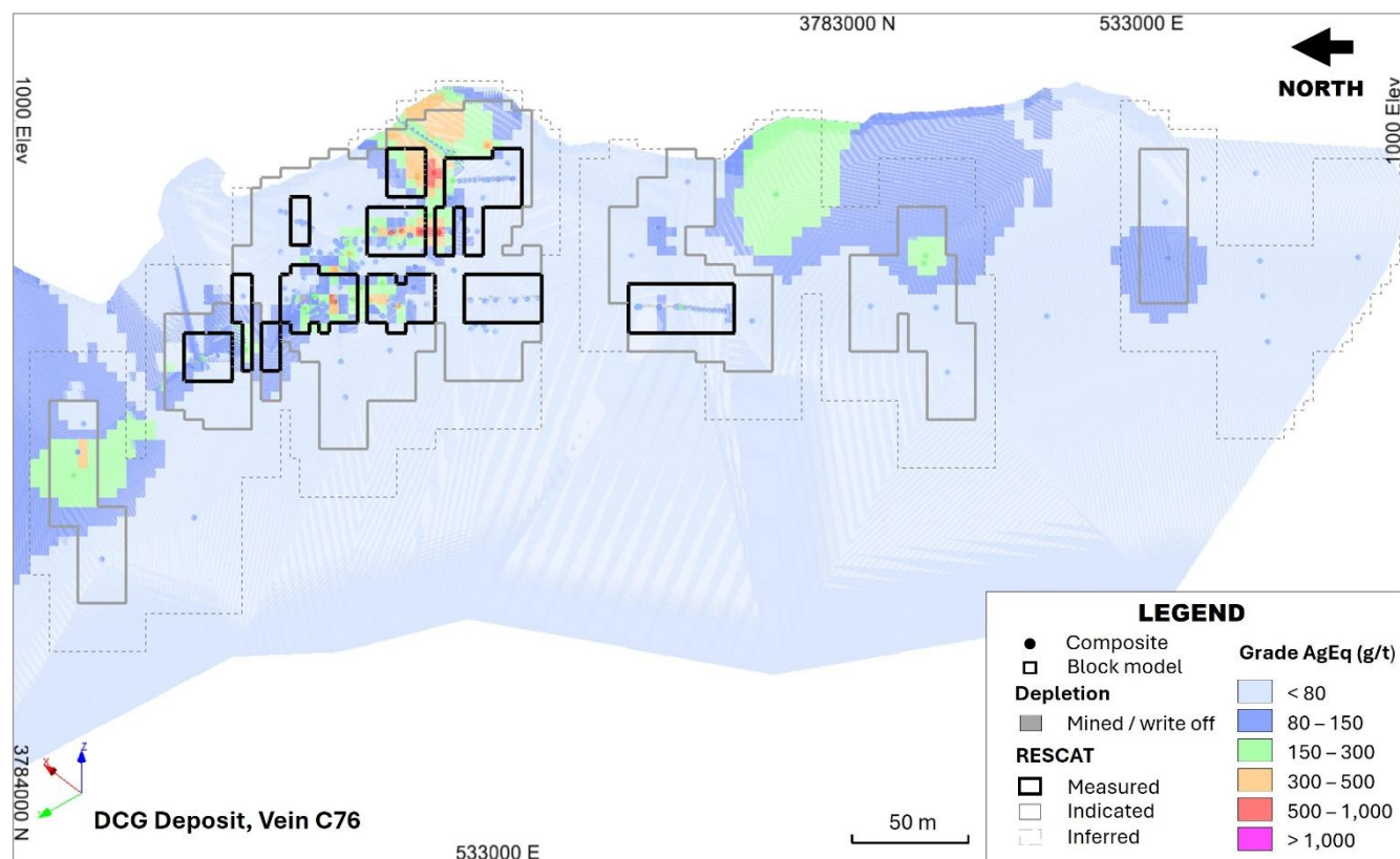
Figure 14.29 DCG - Vein C76 oblique section projection Mineral Resource
