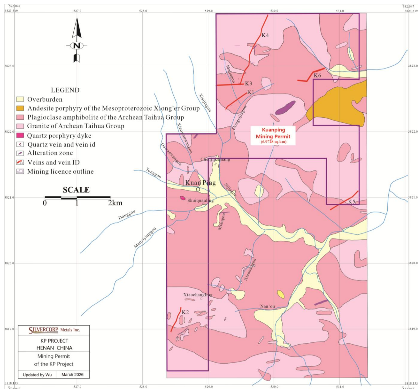
Figure 7.3 KP Project mining licenses and mineralized vein systems
