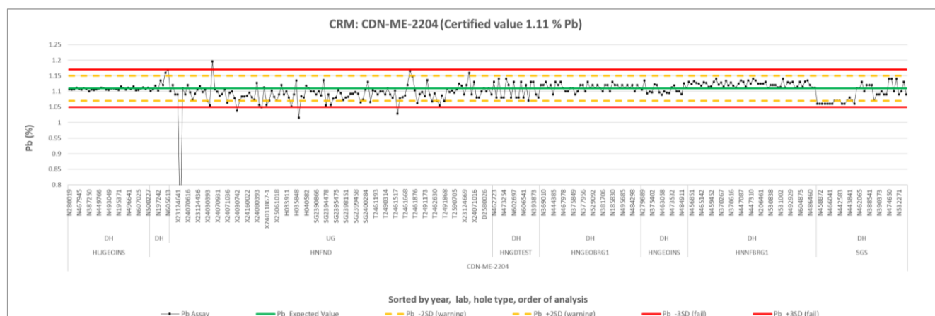
Figure 11.6 Summary control chart for CDN-ME-2204 (Pb)
