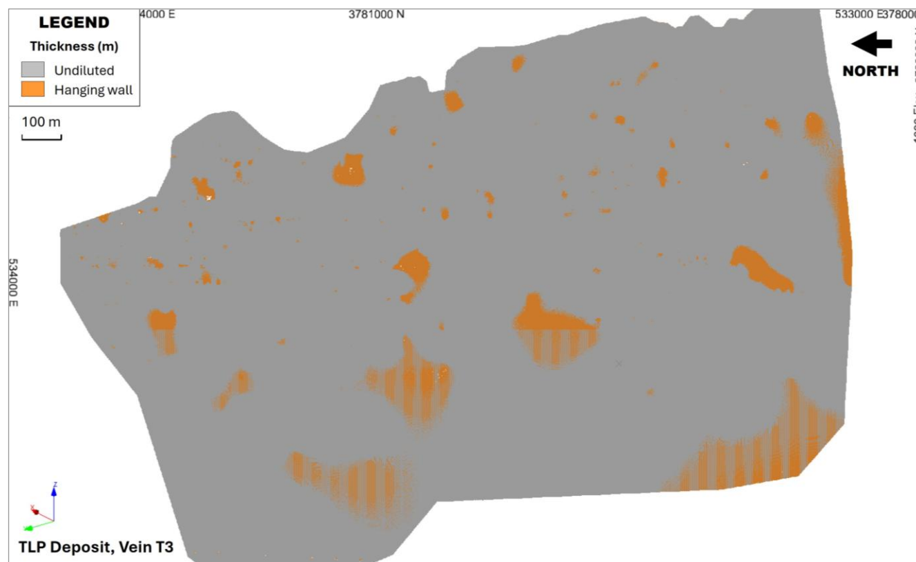
Figure 14.22 TLP_T3 showing the HW dilution that has been added to achieve 0.4 m minimum thickness
