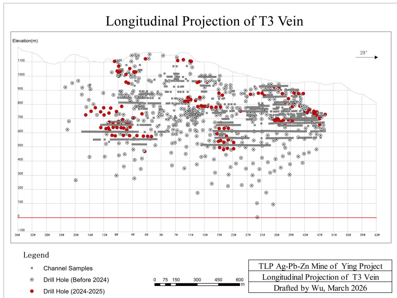
Figure 9.4 Longitudinal projection of Vein T3, TLP
