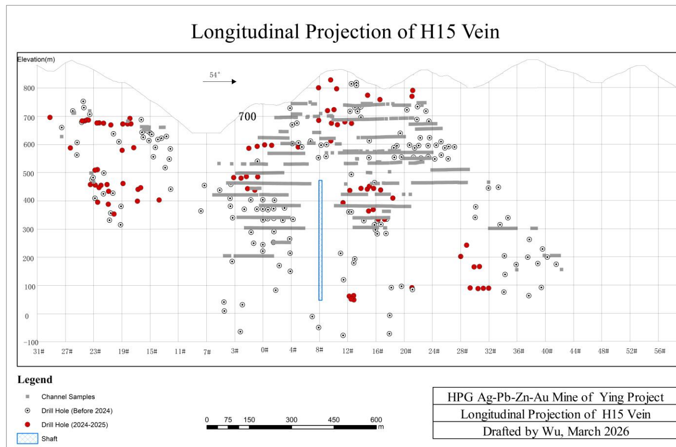
Figure 9.3 Longitudinal projection of Vein H15, HPG
