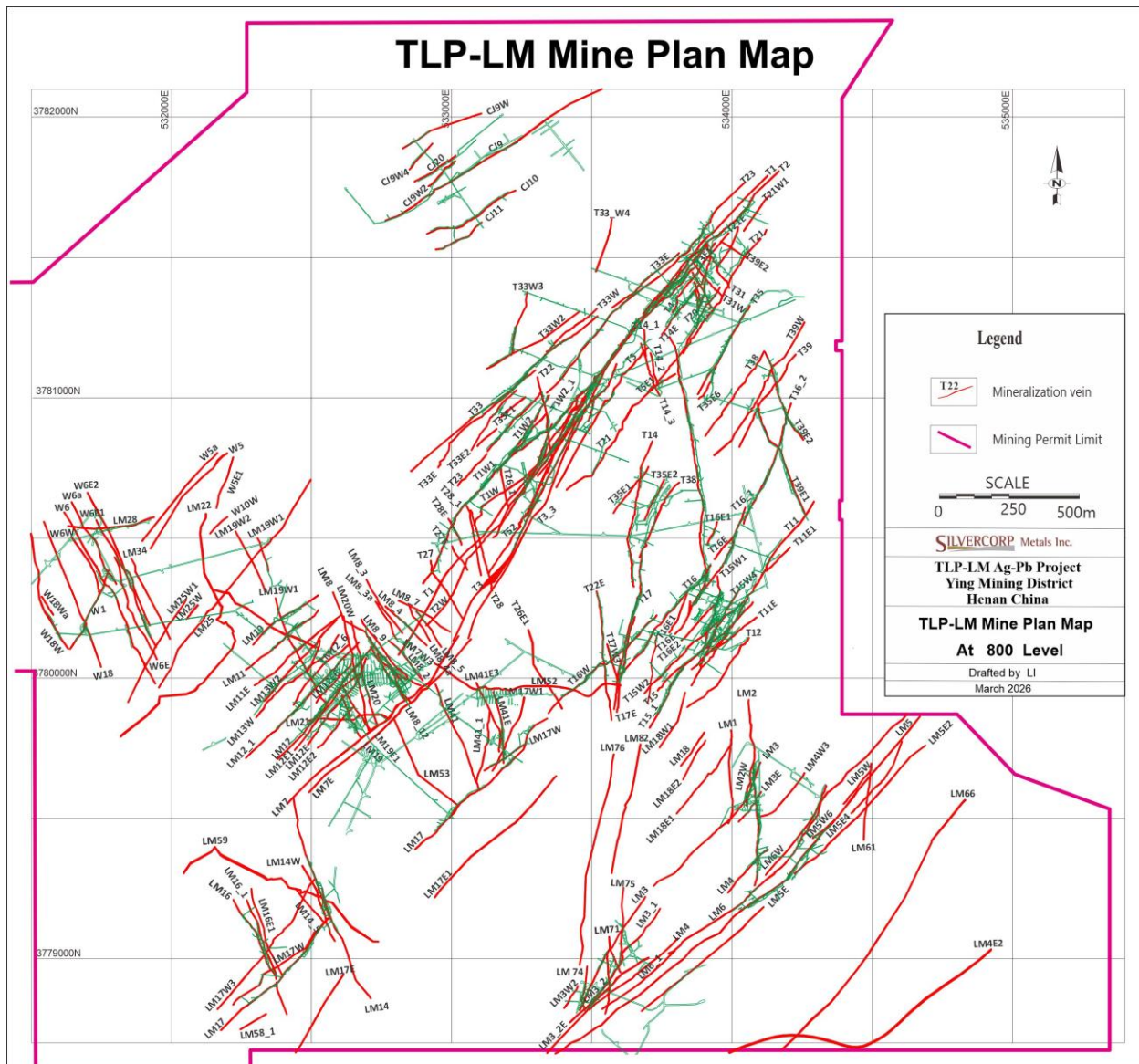
Figure 7.8 Distribution of mineralized veins in the TLP-LM area
