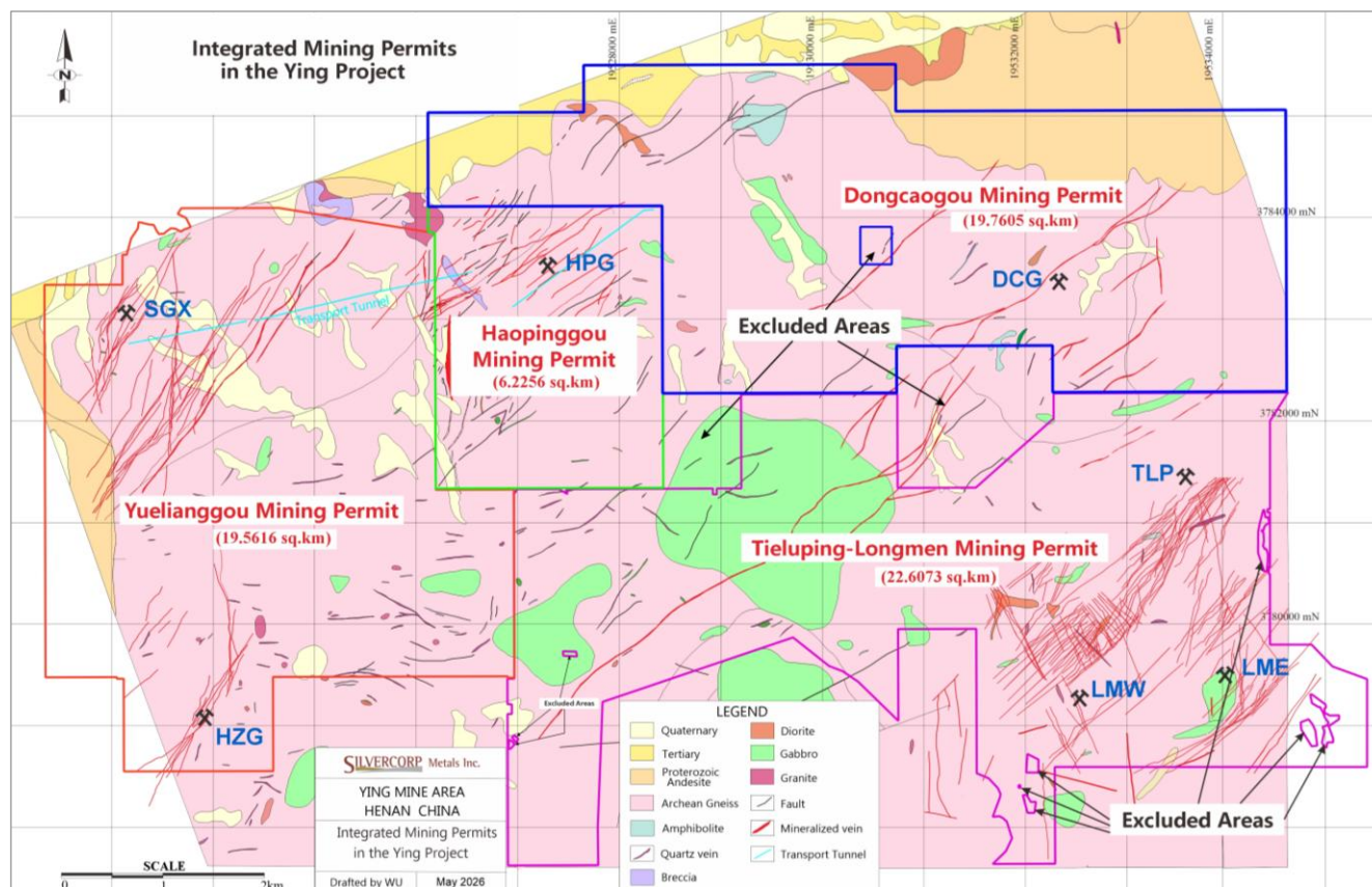
Figure 7.2 Ying Project mining licenses and mineralized vein systems
