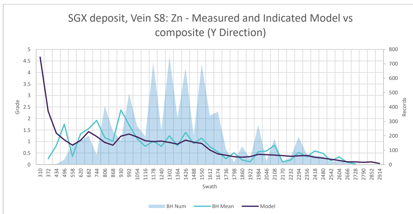
Figure 14.20 S8 zinc swath plot down-dip
