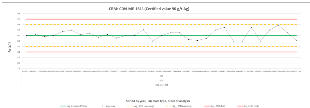
Figure 11.20 Summary control chart for CDN-ME-1811 (Ag)
