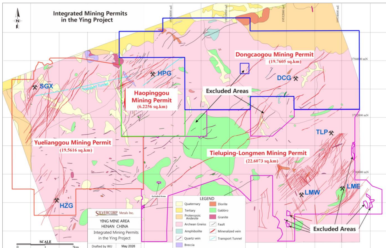
Figure 4.2 Location of the approved mining licenses in the Ying Project
