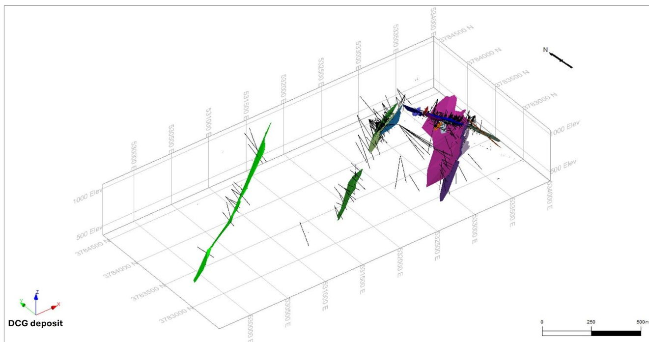
Figure 14.7 3D view of the DCG mineralization wireframes
