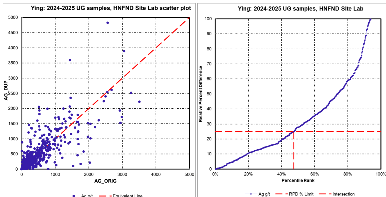
Figure 11.14 Ying field duplicate RPD and scatter plots of Ag (channel samples)
