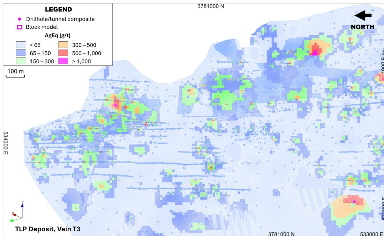
Figure 14.14 Silver equivalent grade longitudinal projection TLP mine: Vein T3
