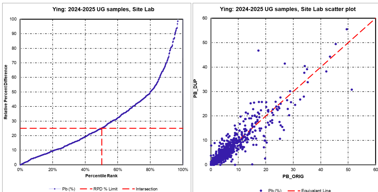
Figure 11.15 Ying field duplicate RPD and scatter plots of Pb (channel samples)
