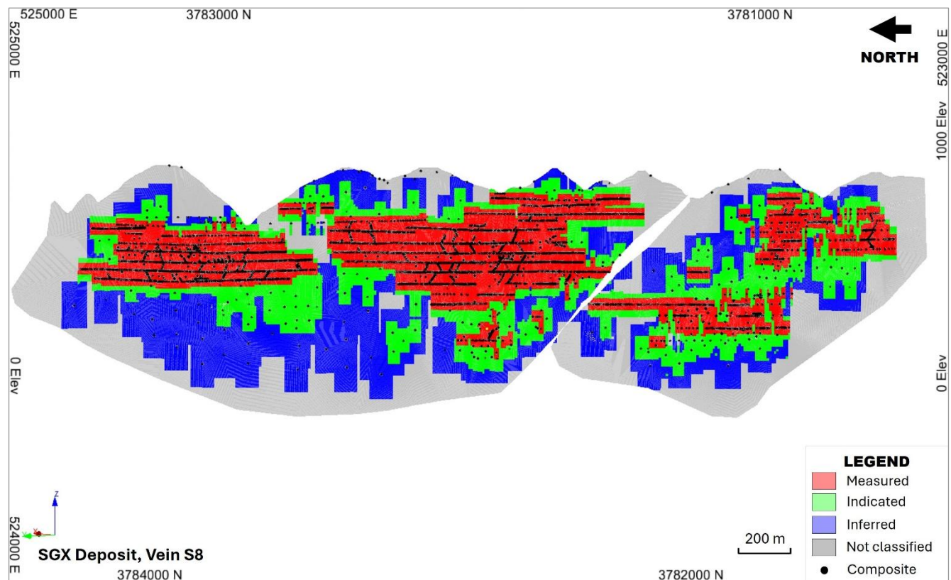
Figure 14.12 Mineral Resource classification longitudinal projection SGX mine: Vein S8
