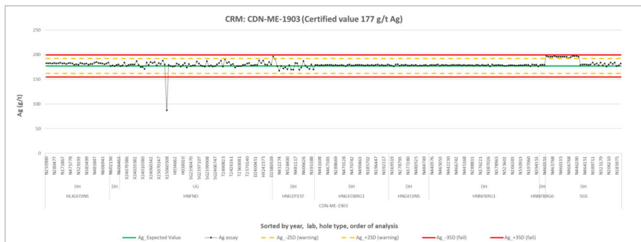
Figure 11.4 Summary control chart for CDN-ME-1903 (Ag)
