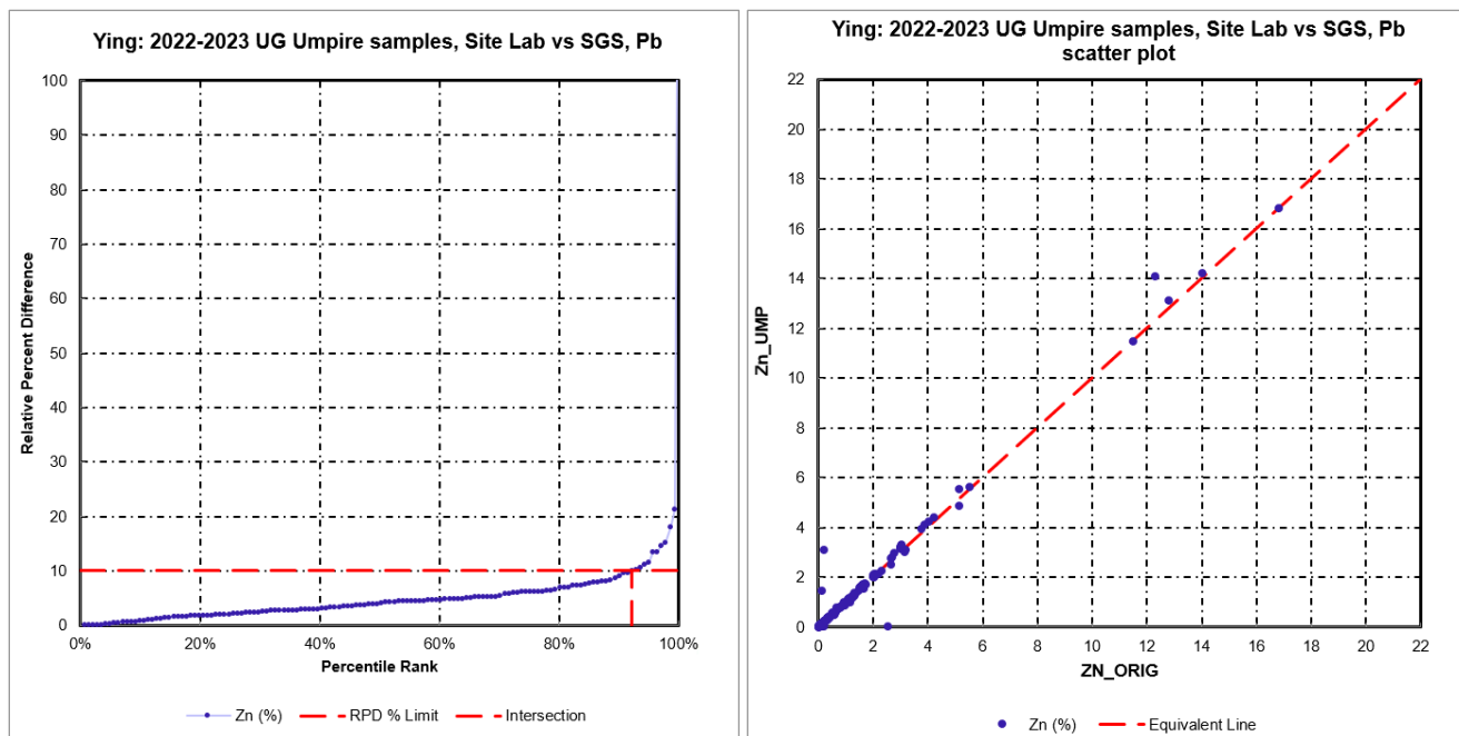
Figure 11.19 Ying umpire RPD and scatter plots of Zn (UG samples, Site Lab, SGS Umpire Lab)
