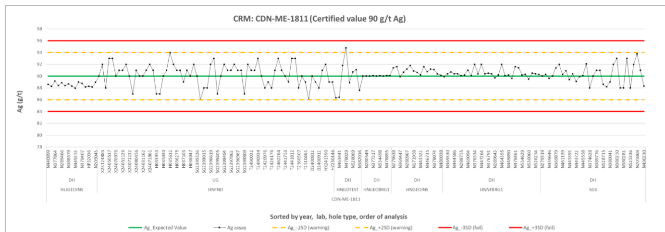
Figure 11.3 Summary control chart for CDN-ME-1811 (Ag)
