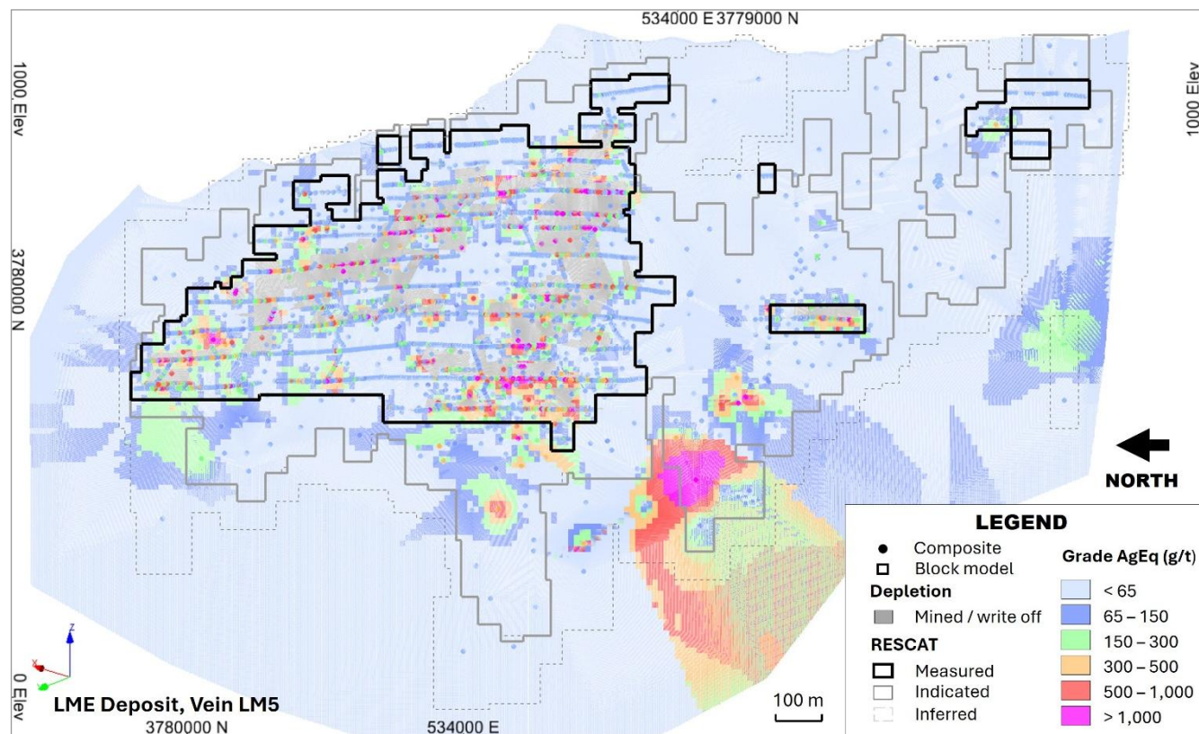
Figure 14.27 LME - Vein LM5 vertical long section projection Mineral Resource
