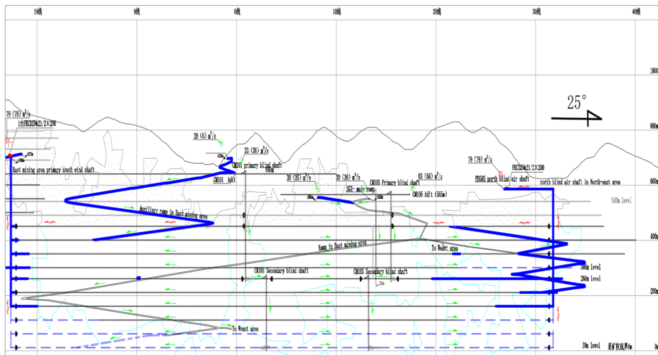
Figure 16.13 SGX ventilation system diagram looking North 65° West
