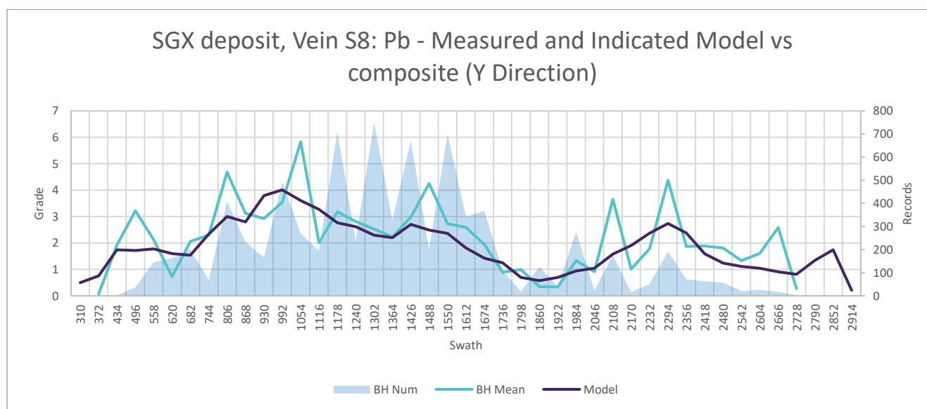
Figure 14.18 S8 lead swath plot down-dip
