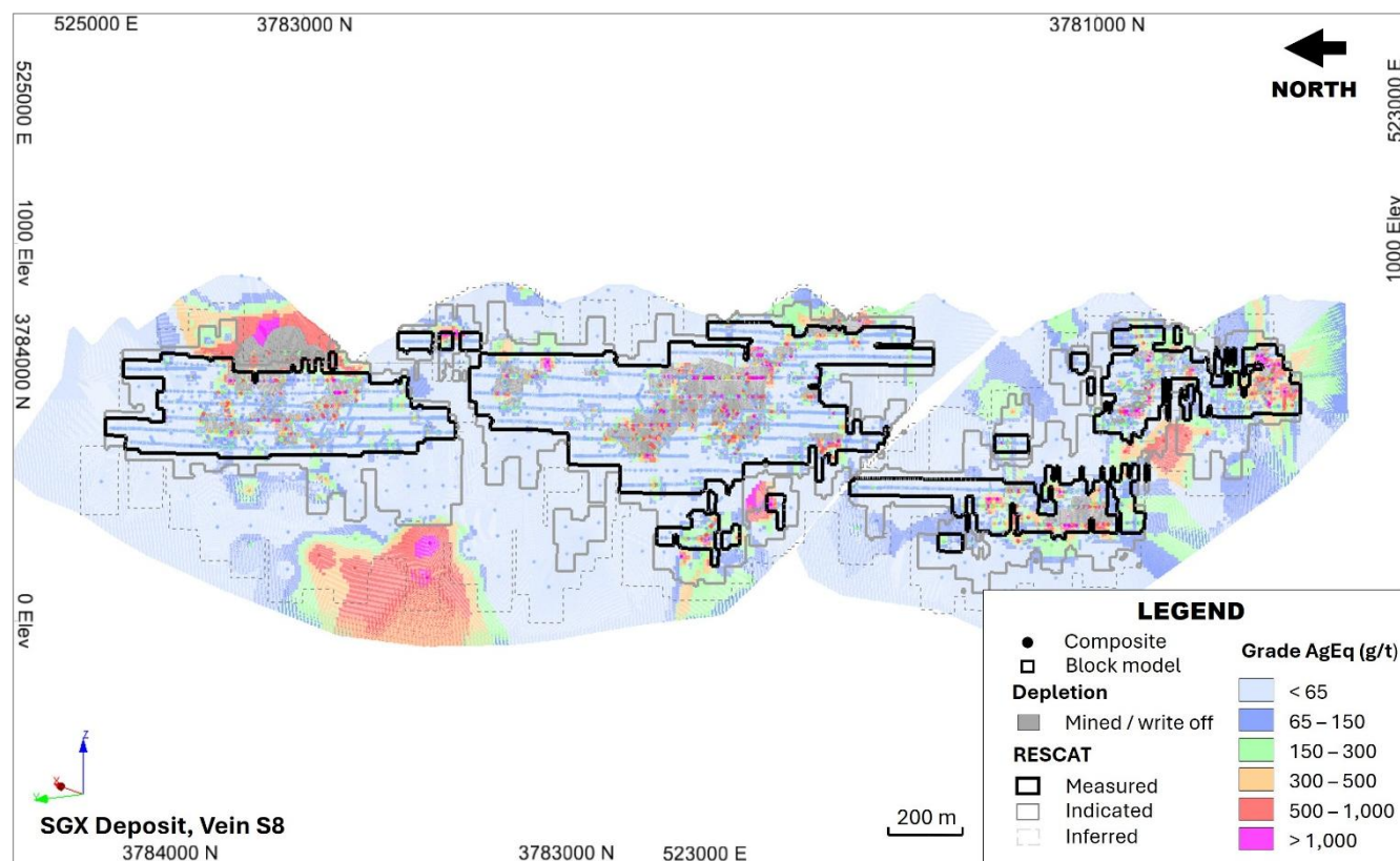
Figure 14.23 SGX - Vein S8 vertical long section projection Mineral Resource
