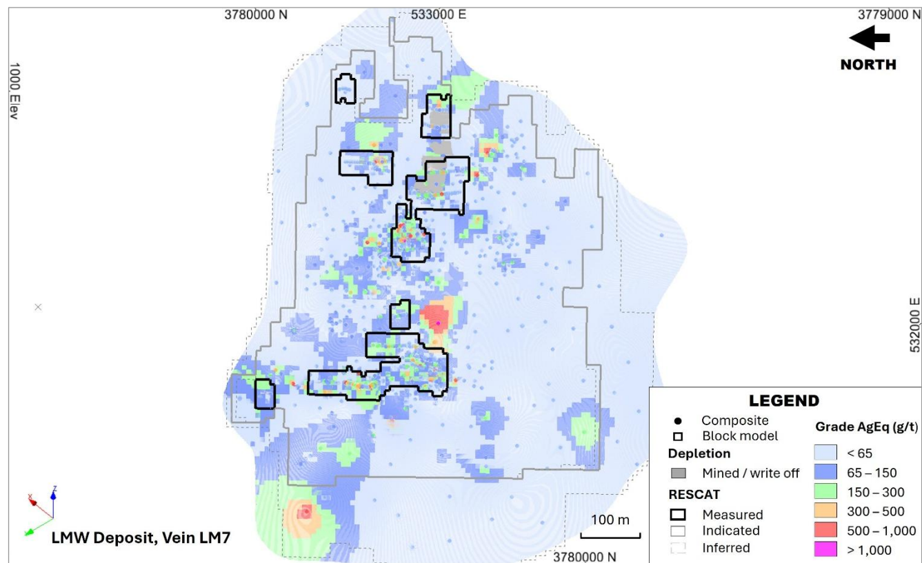
Figure 14.28 LMW - Vein LM7 vertical long section projection Mineral Resource
