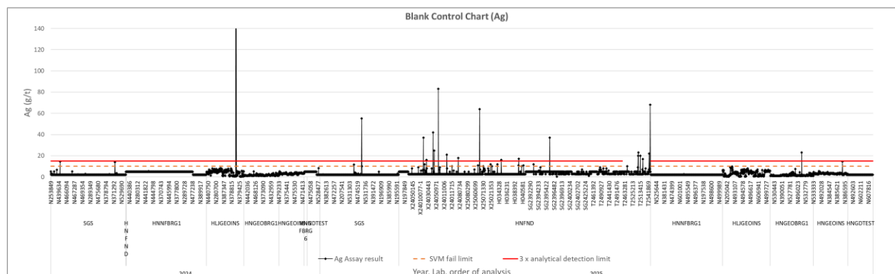
Figure 11.11 Coarse blank control chart (Ag)
