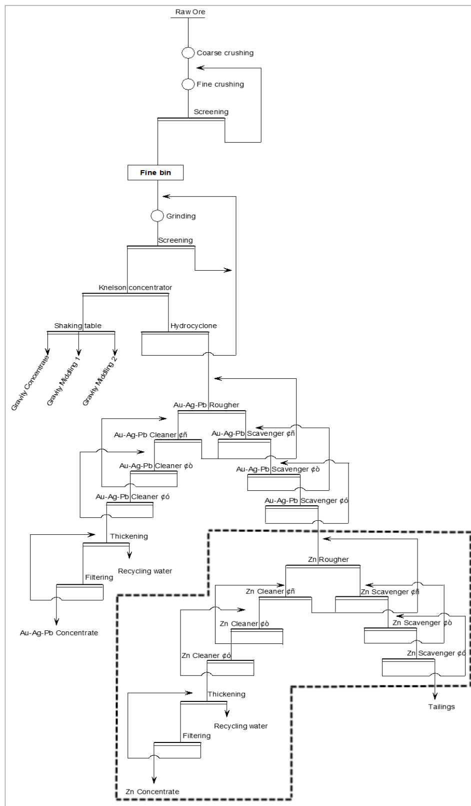
Figure 17.4 Flowsheet (Plant 1)
