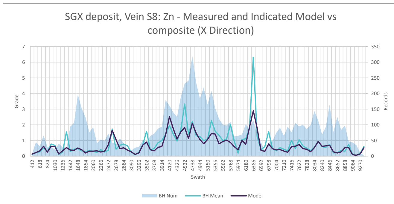
Figure 14.19 S8 zinc swath plot along strike
