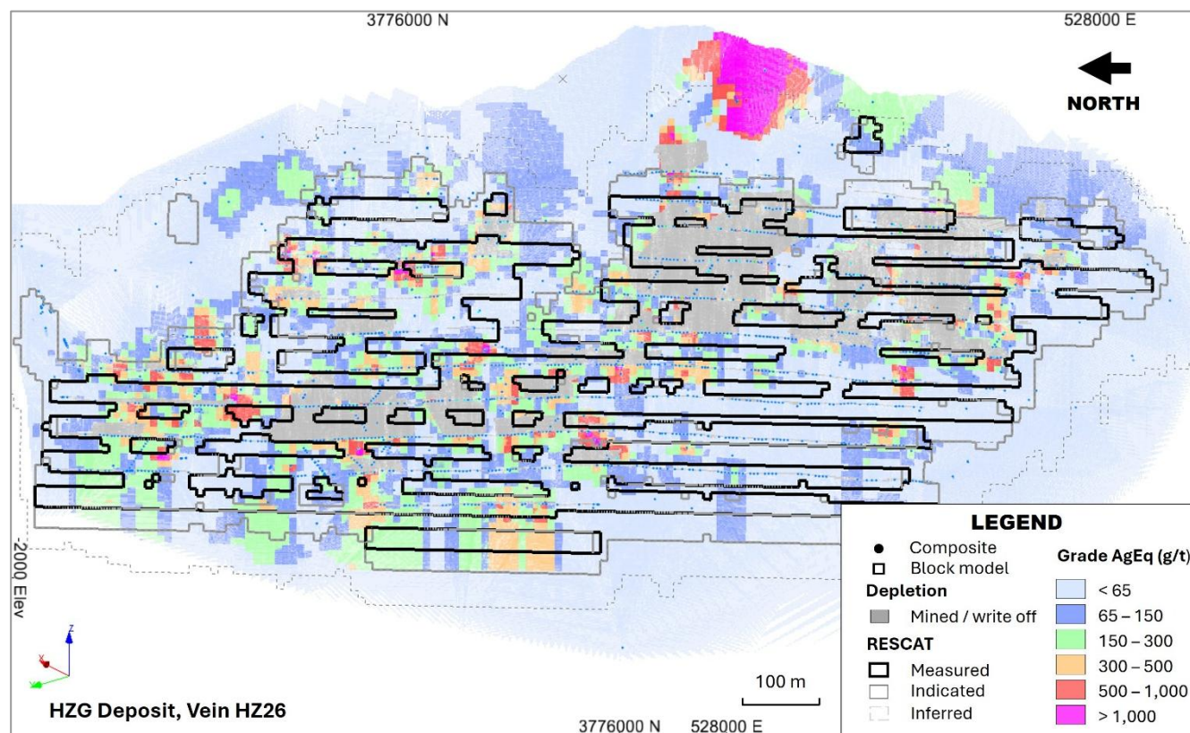
Figure 14.24 HZG - Vein HZ26 vertical long section projection Mineral Resource
