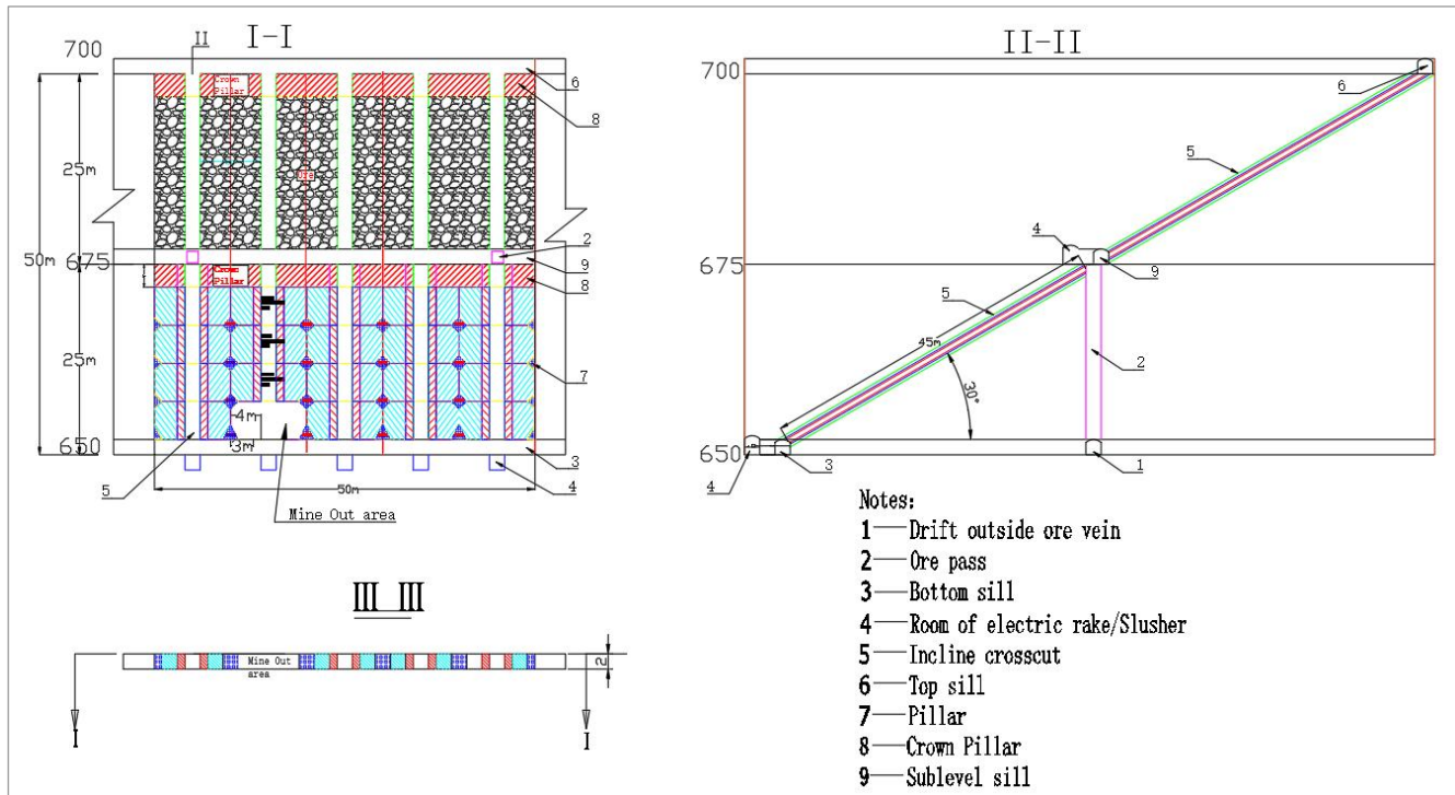
Figure 16.10 Room and pillar mining method
