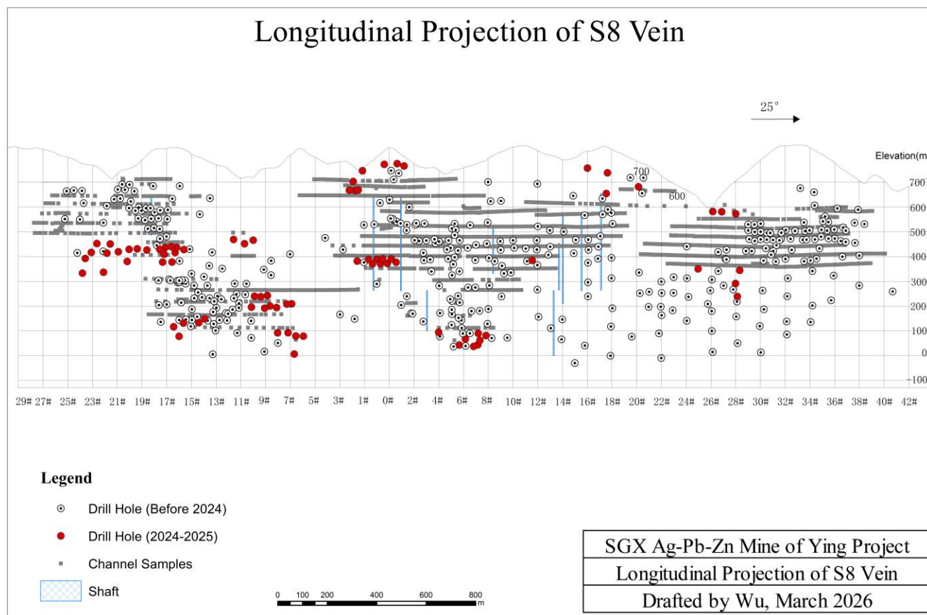
Figure 9.1 Longitudinal projection of Vein S8, SGX
