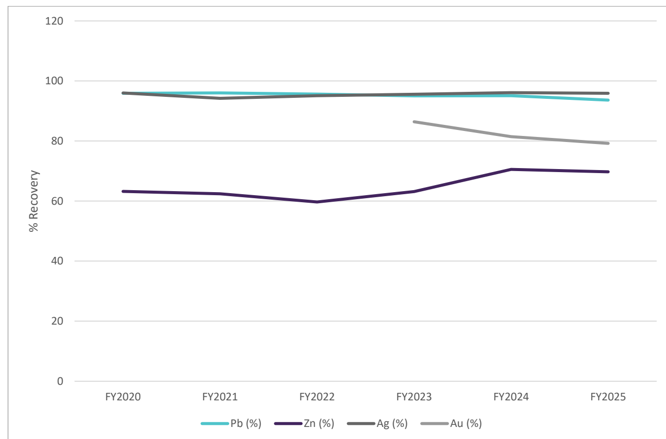
Figure 17.2 Overall metal recovery to concentrate - FY2020 to FY2025
