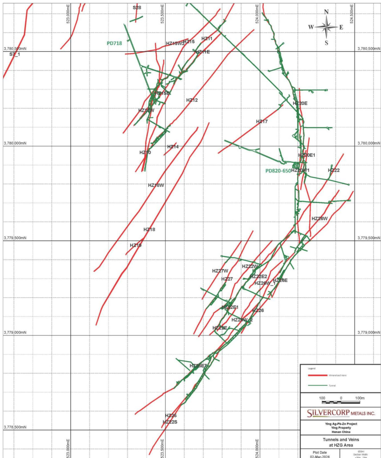
Figure 7.6 Tunnels and veins in the HZG area
