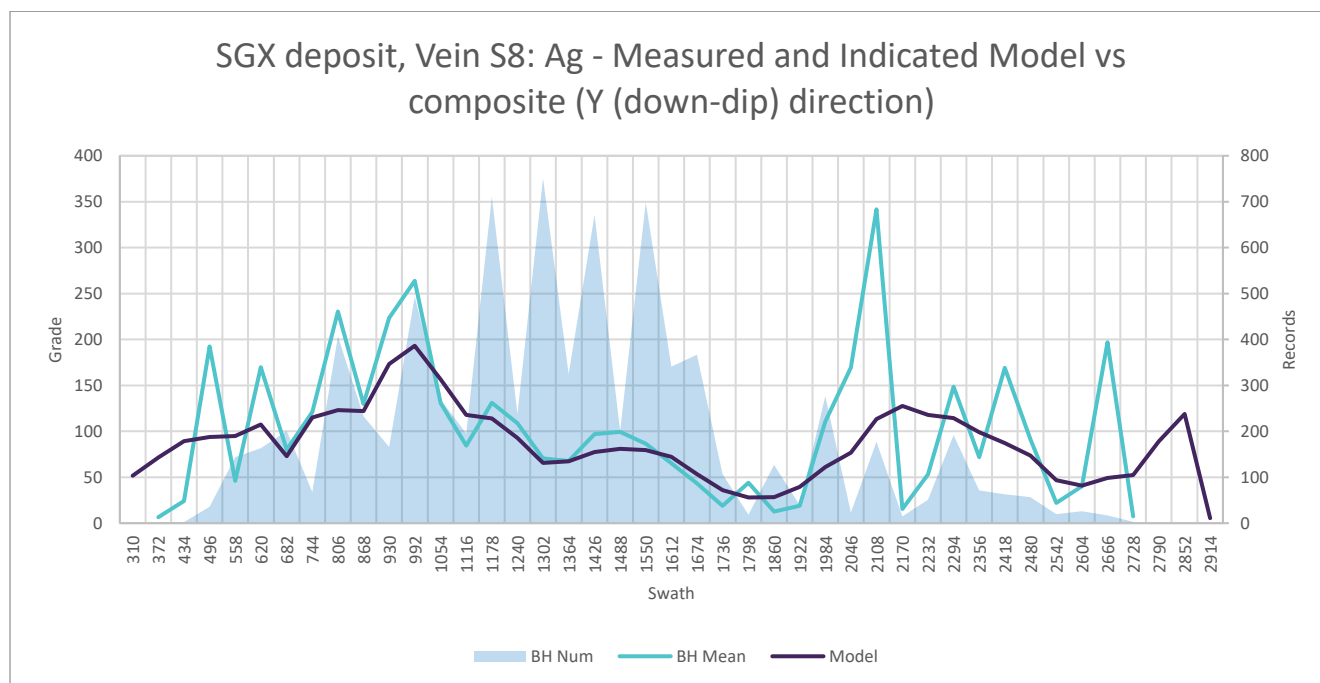
Figure 14.16 S8 silver swath plot down-dip
