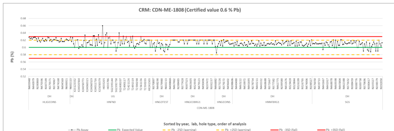
Figure 11.5 Summary control chart for CDN-ME-1808 (Pb)
