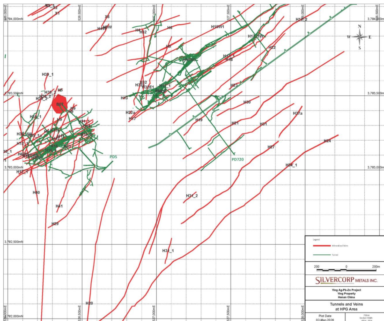
Figure 7.7 Tunnels and veins in the HPG area
