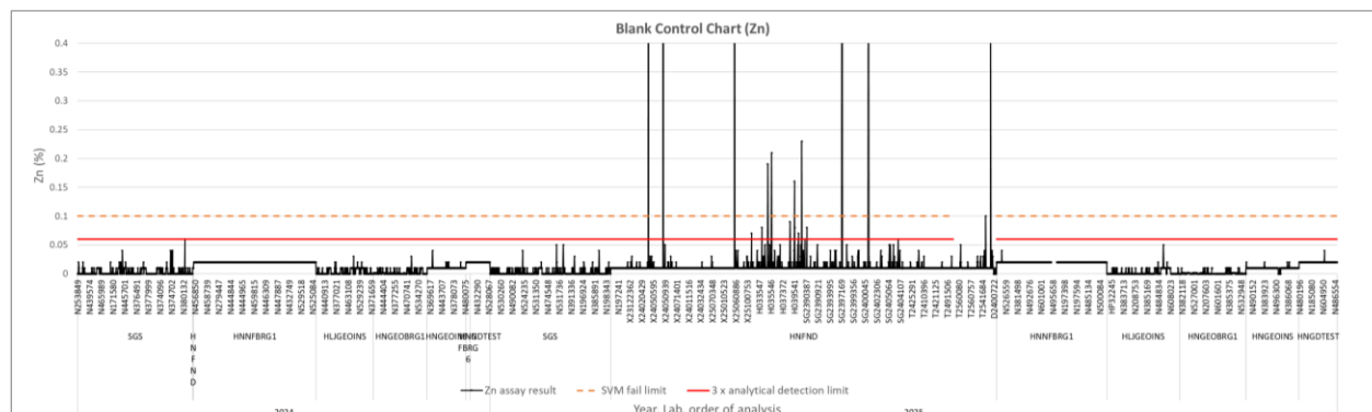
Figure 11.13 Coarse blank control chart (Zn)
