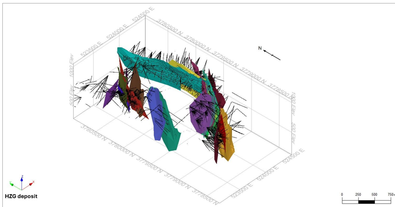
Figure 14.2 3D view of the HZG mineralization wireframes
