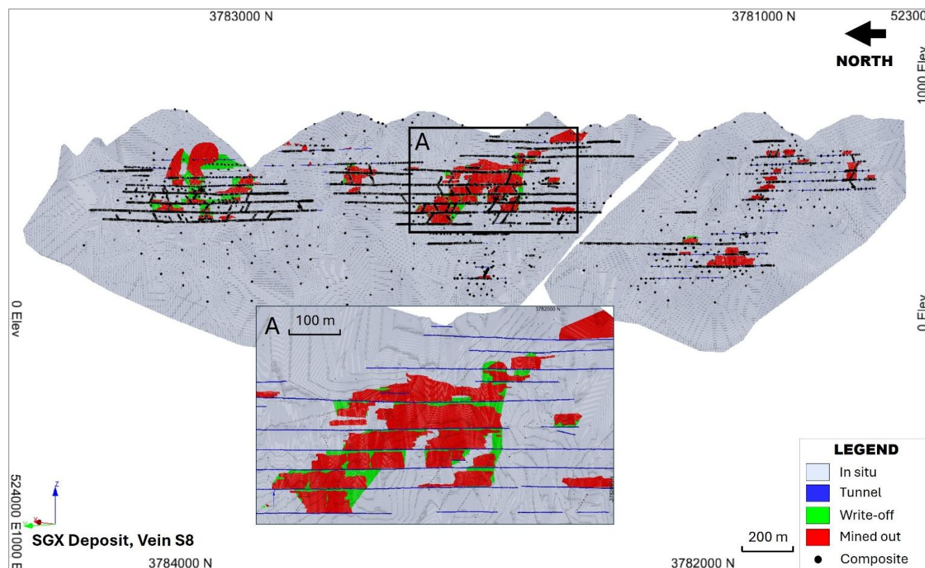
Figure 14.11 Mining depletion longitudinal projection SGX mine: Vein S8
