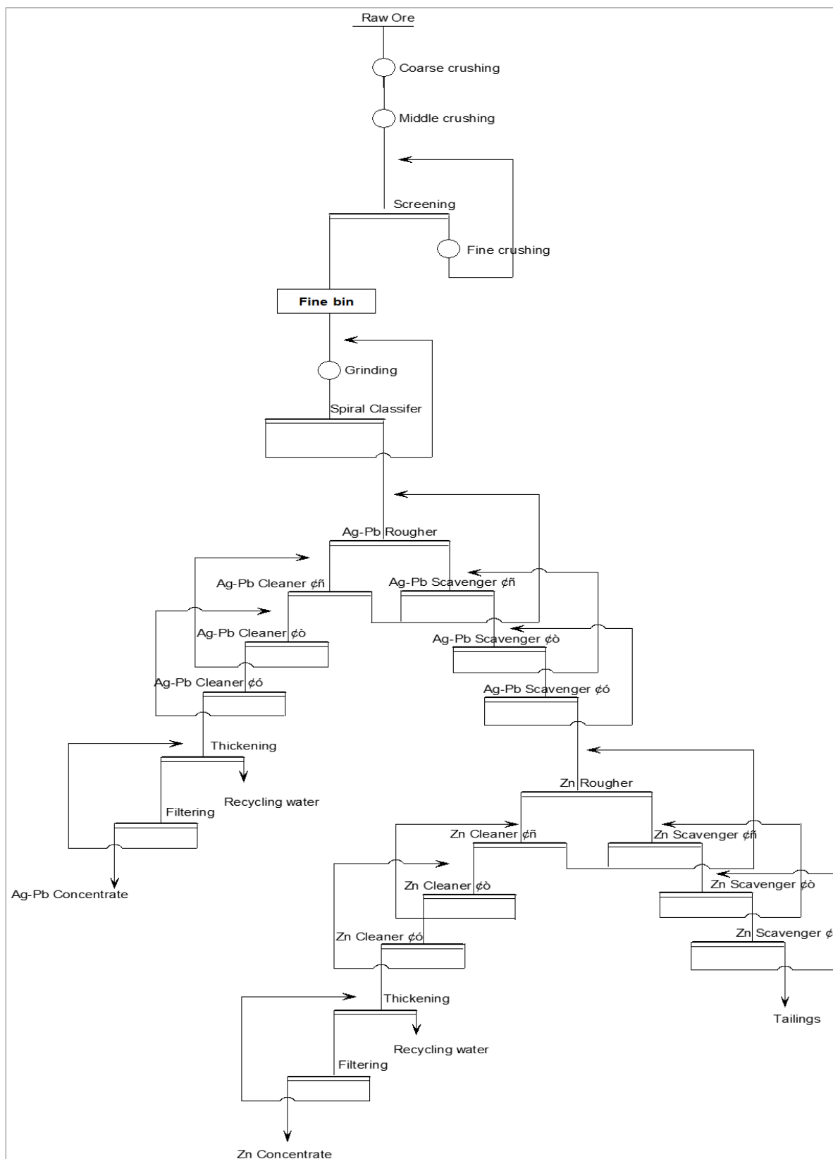
Figure 17.6 Flowsheet for Plant 2
