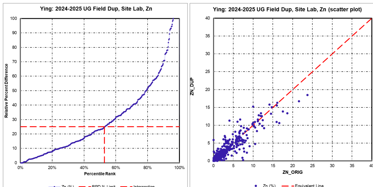
Figure 11.16 Ying field duplicate RPD and scatter plots of Zn (channel samples)
