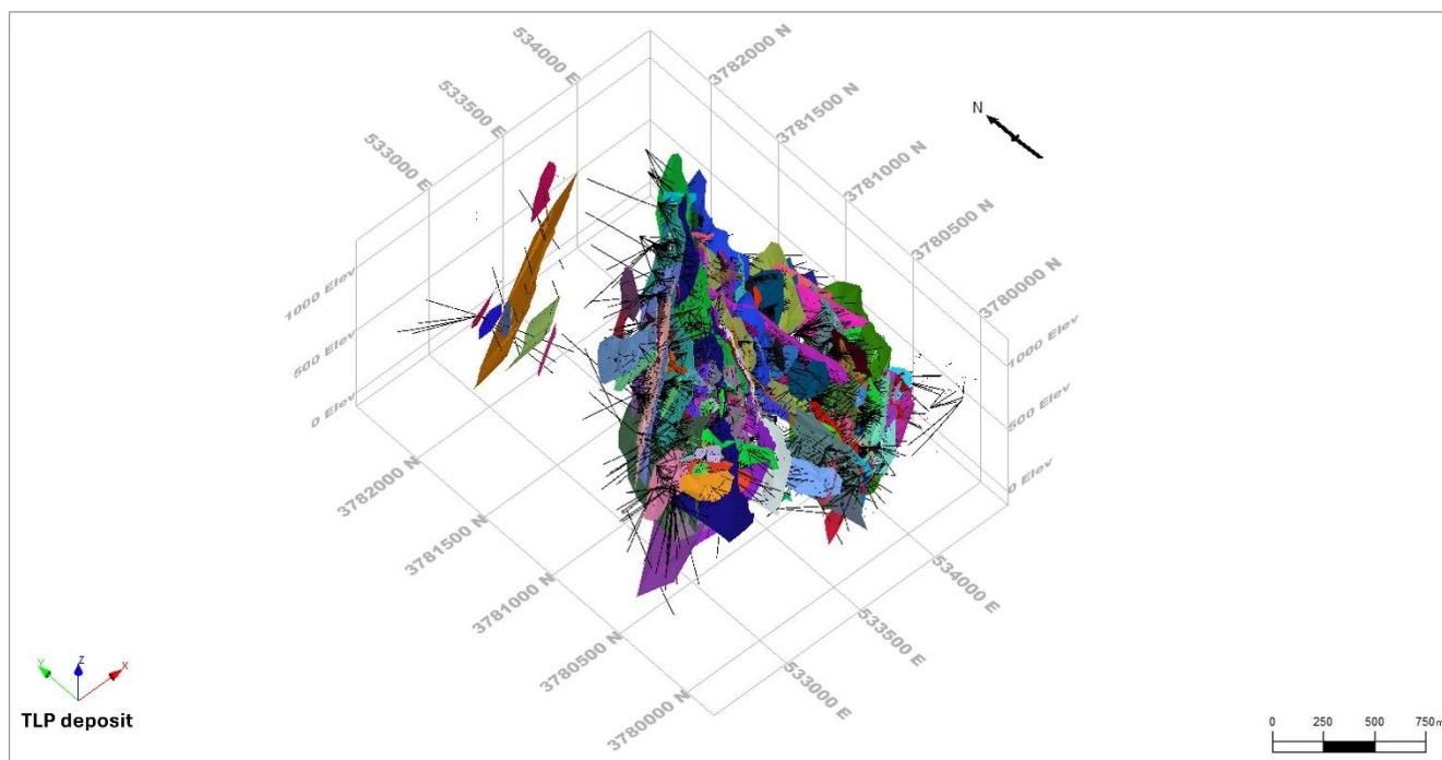
Figure 14.4 3D view of the TLP mineralization wireframes
