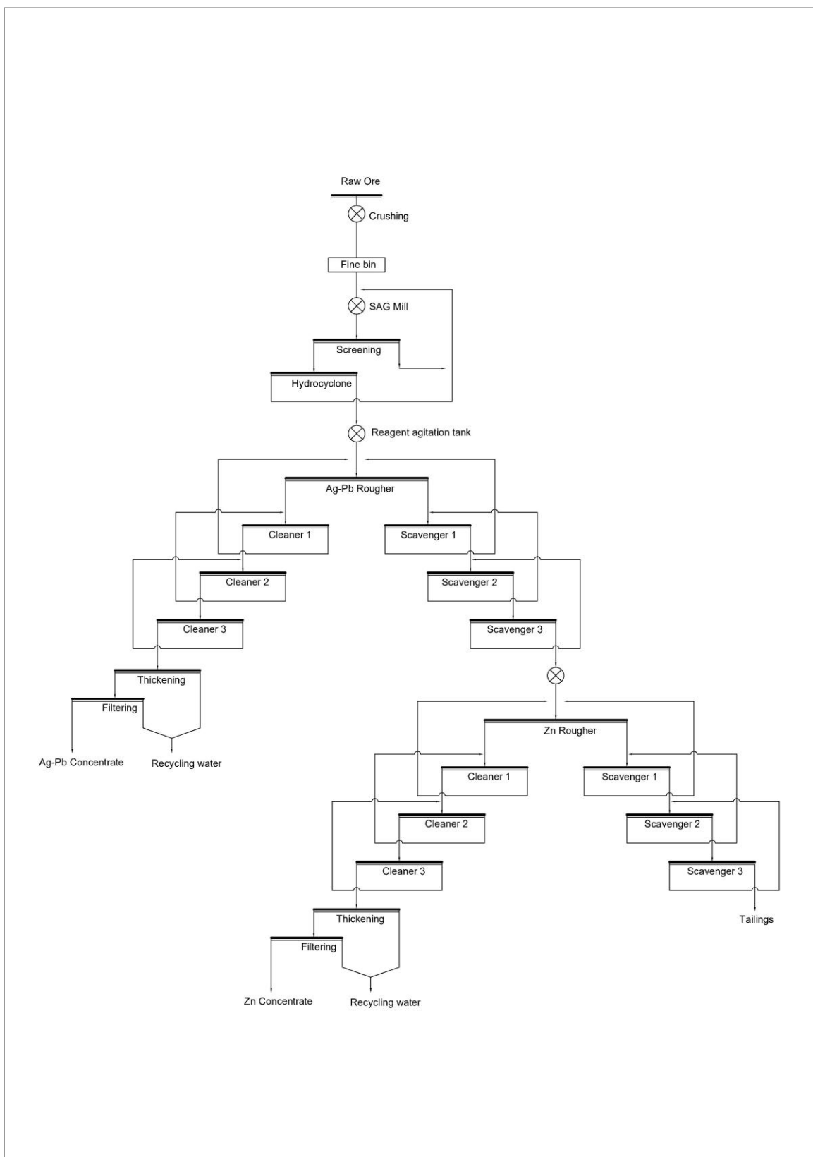
Figure 17.7 Flowsheet for Plant 3
