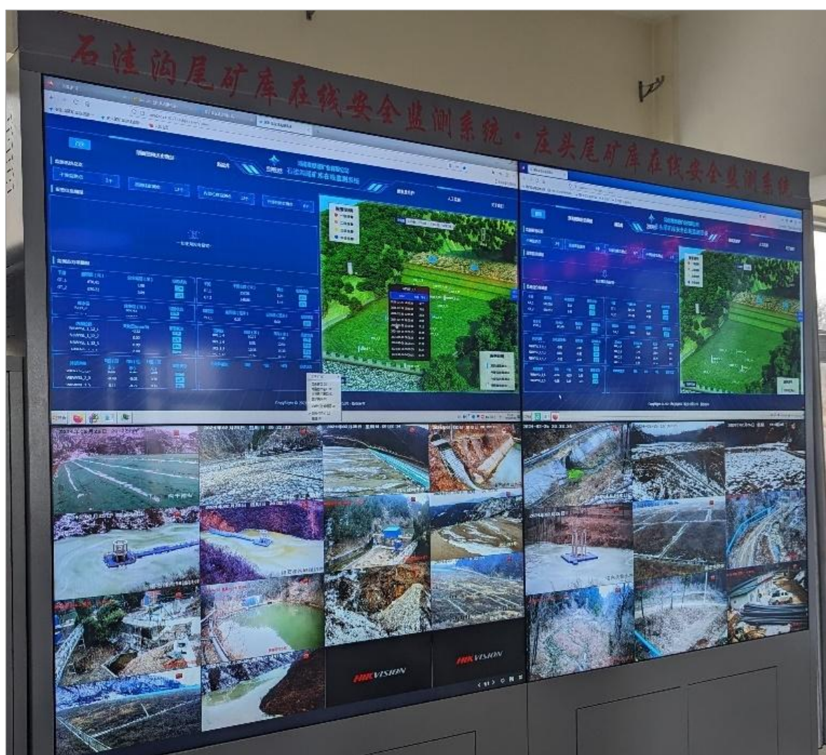
Figure 18.9 TSF monitoring data displayed in the control room
