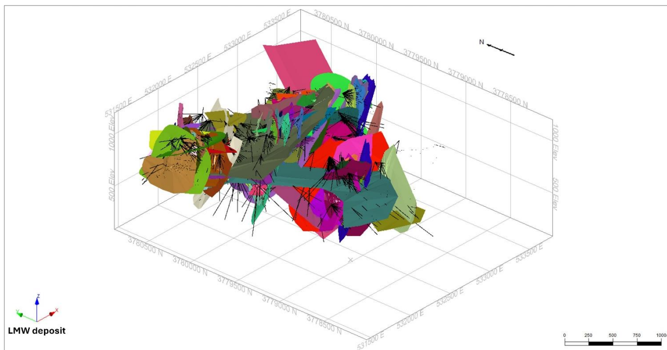
Figure 14.6 3D view of the LMW mineralization wireframes
