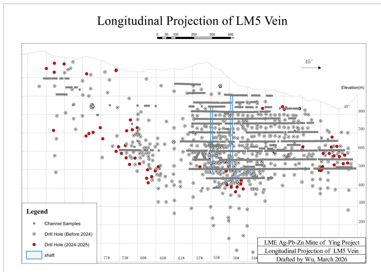
Figure 9.5 Longitudinal projection of Vein LM5, LME
