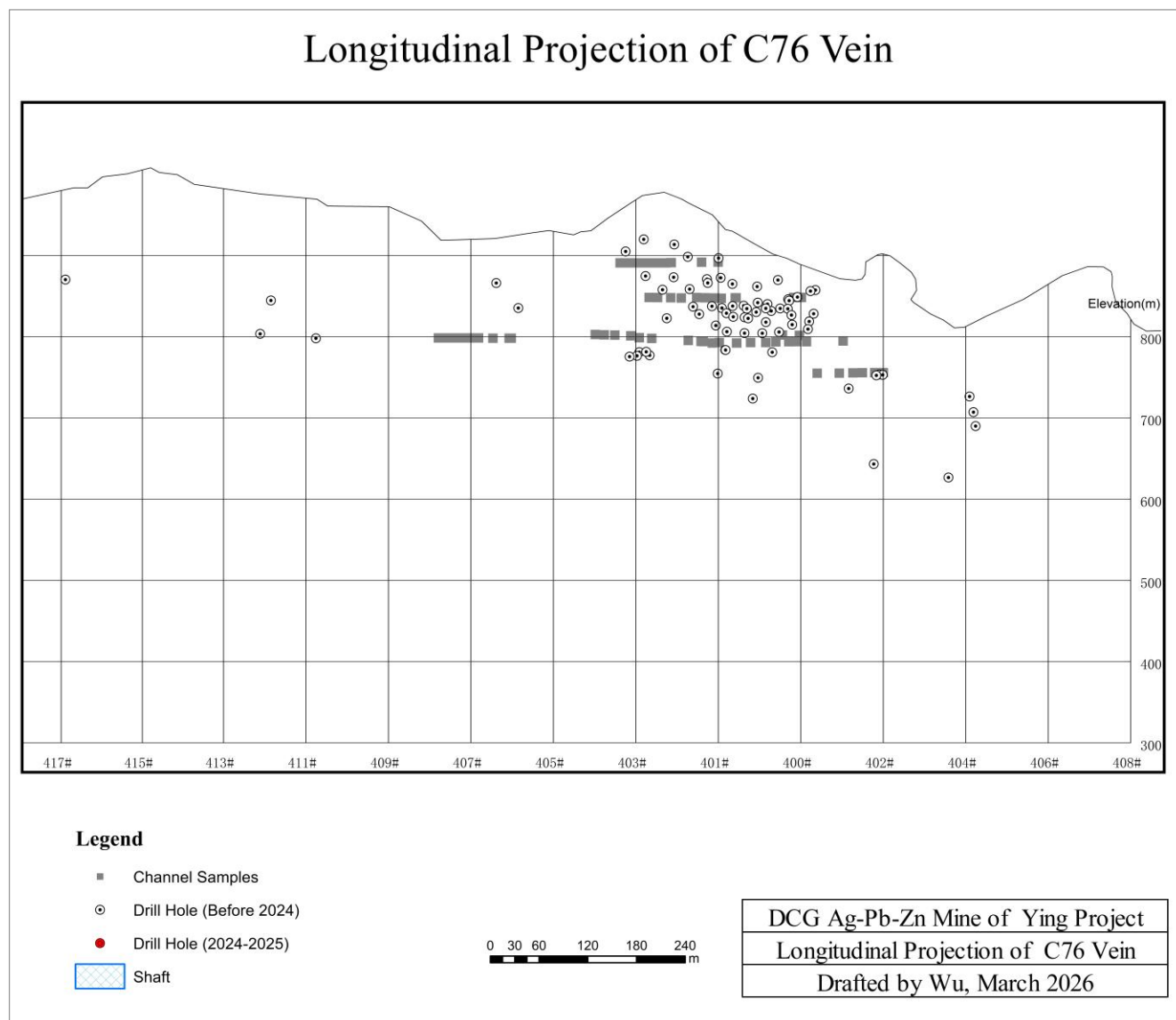
Figure 9.7 Longitudinal projection of Vein C76, DCG
