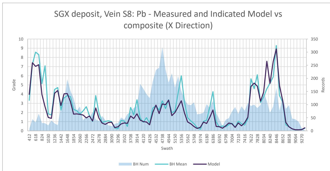
Figure 14.17 S8 lead swath plot along strike
