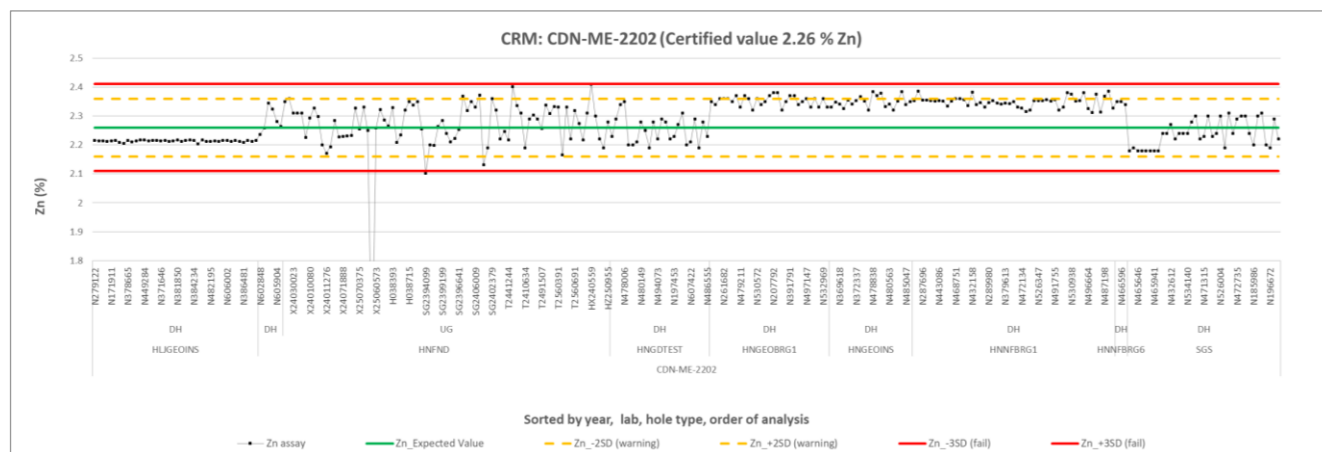
Figure 11.9 Summary control chart for CDN-ME-2202 (Zn)
