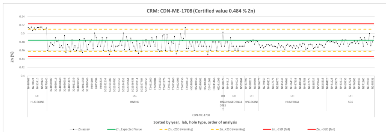
Figure 11.7 Summary control chart for CDN-ME-1708 (Zn)
