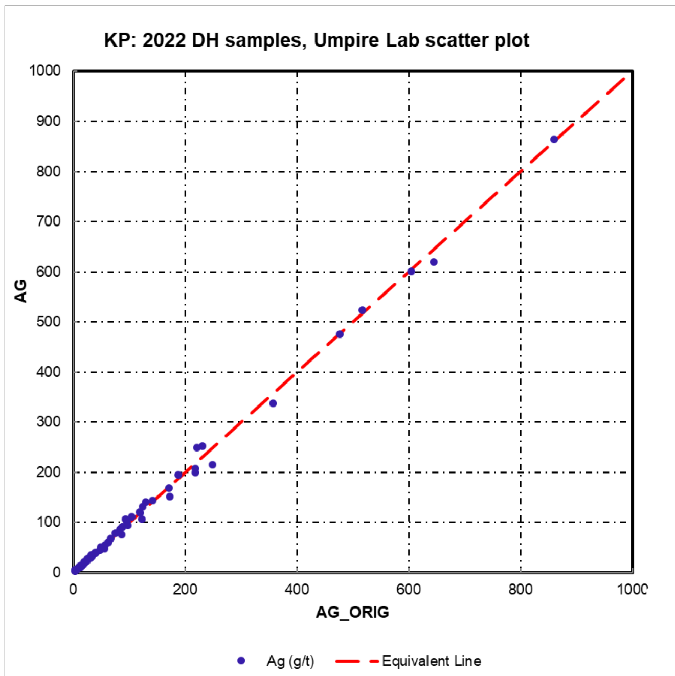
Figure 11.23 KP Project – 2022 drilling umpire scatter plot
