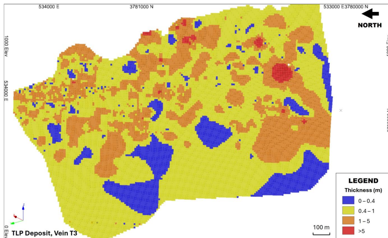
Figure 14.21 Vein thickness of the TLP_T3 vein
