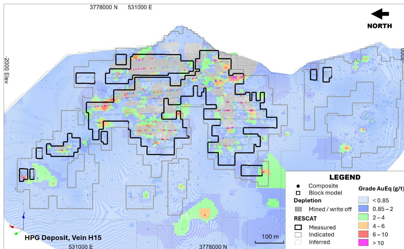
Figure 14.25 HPG - Vein H15 vertical long section projection Mineral Resource
