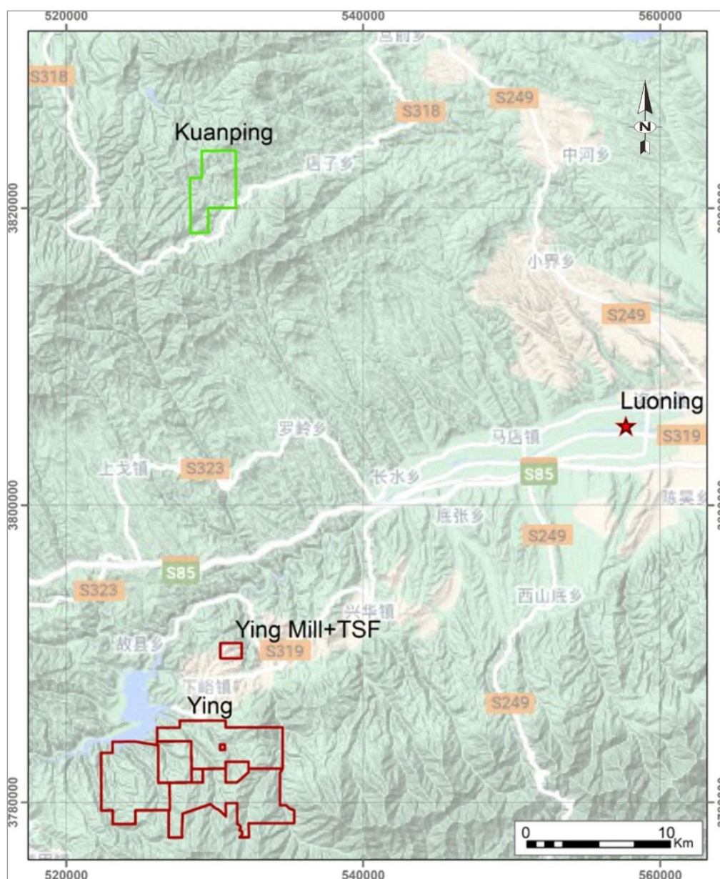
Figure 16.1 Ying Property mines locations
