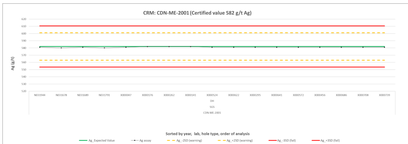
Figure 11.21 Summary control chart for CDN-ME-2001 (Ag)
