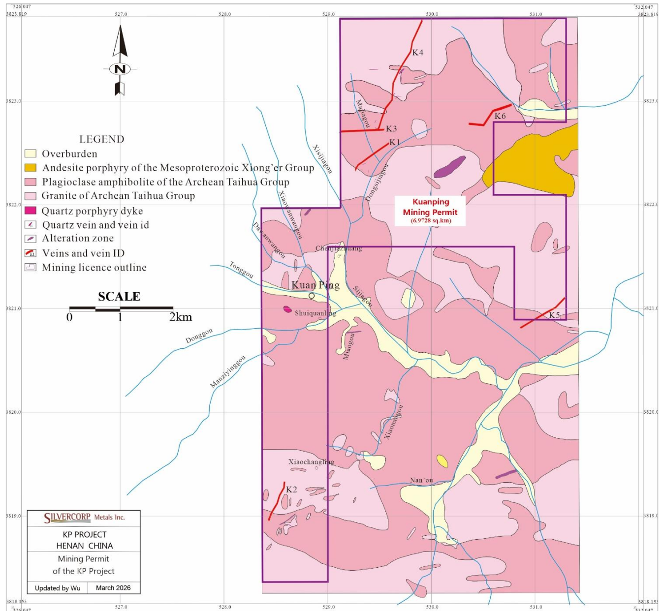
Figure 4.3 Location of approved mining license for KP Project
