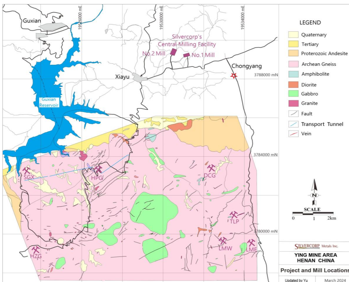
Figure 5.1 Ying Project mine and mill locations
