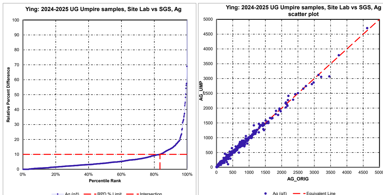
Figure 11.17 Ying umpire RPD and scatter plots of Ag (UG samples, Site Lab, SGS Umpire Lab)
