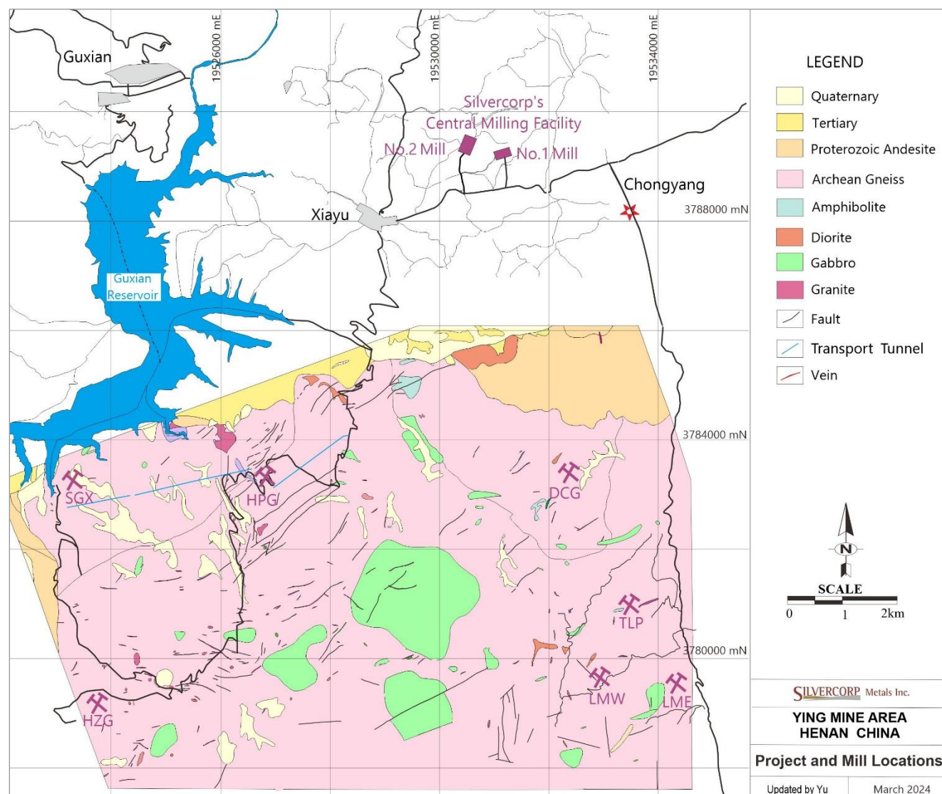
Figure 16.2 Ying Project mine and mill locations
