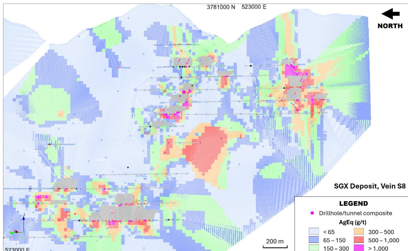
Figure 14.13 Silver equivalent grade longitudinal projection SGX mine: Vein S8
