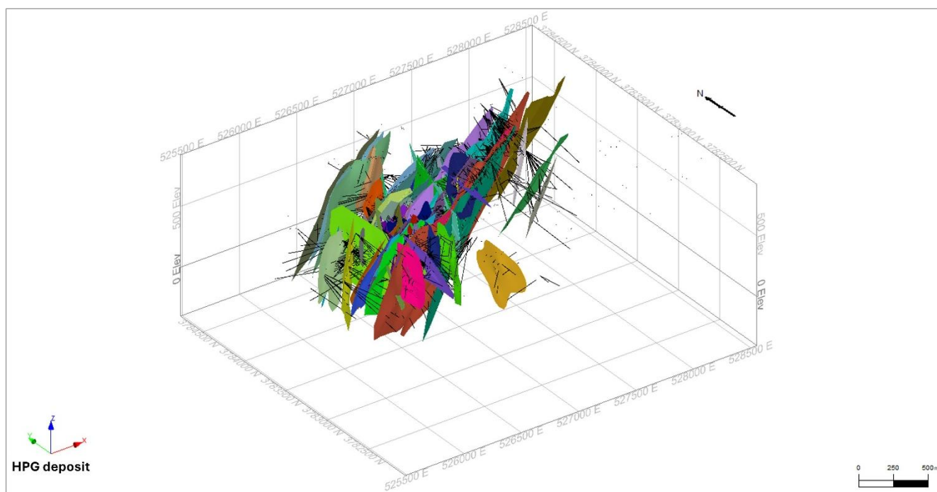
Figure 14.3 3D view of the HPG mineralization wireframes
