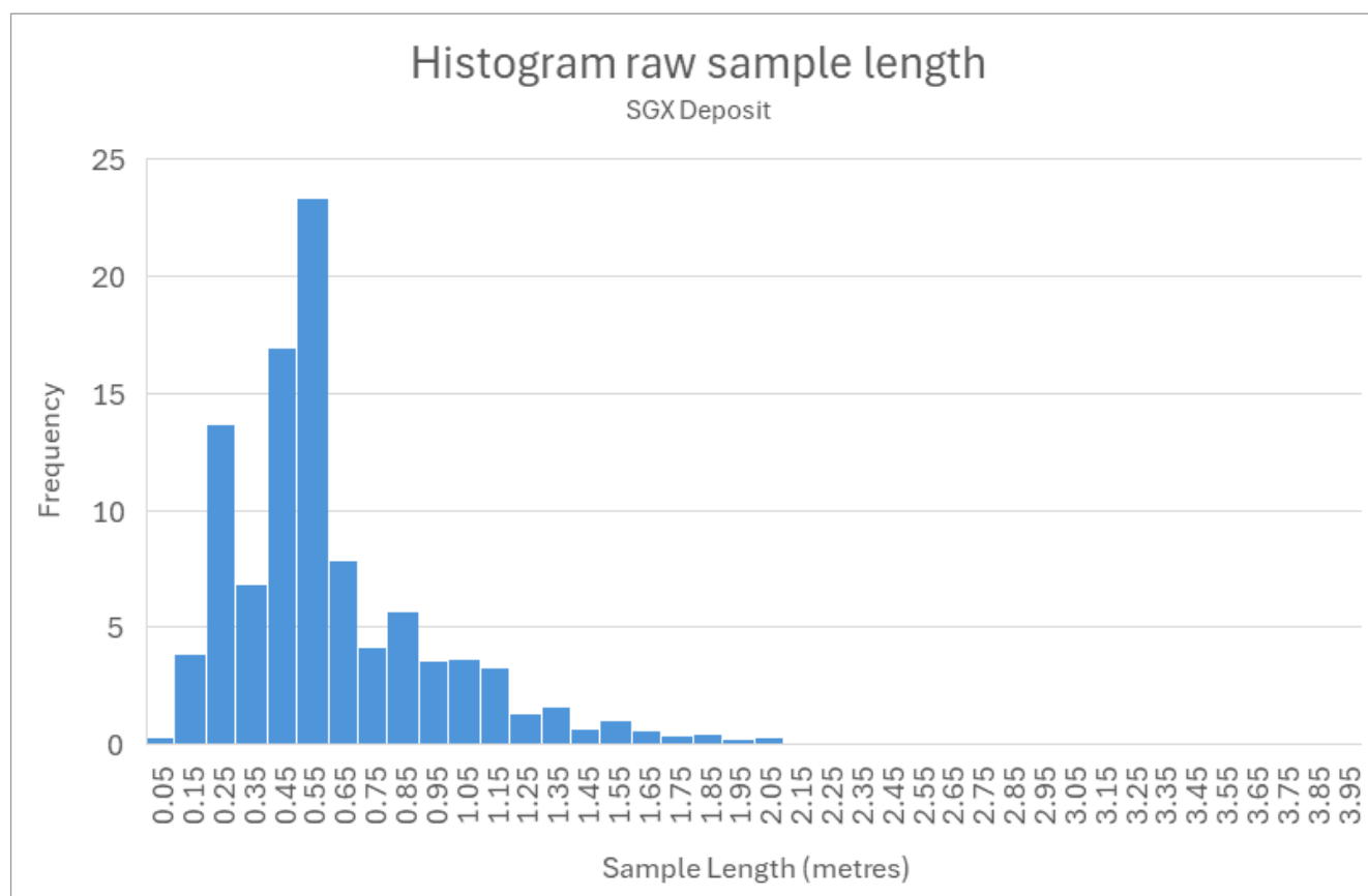
Figure 14.9 SGX mineralized sample length histogram
