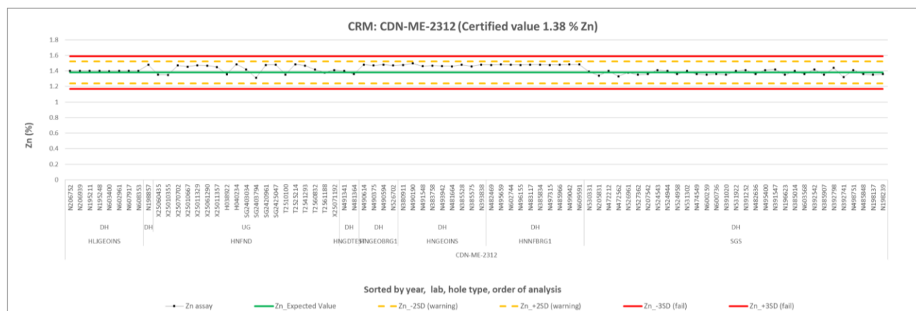
Figure 11.8 Summary control chart for CDN-ME-2312 (Zn)
