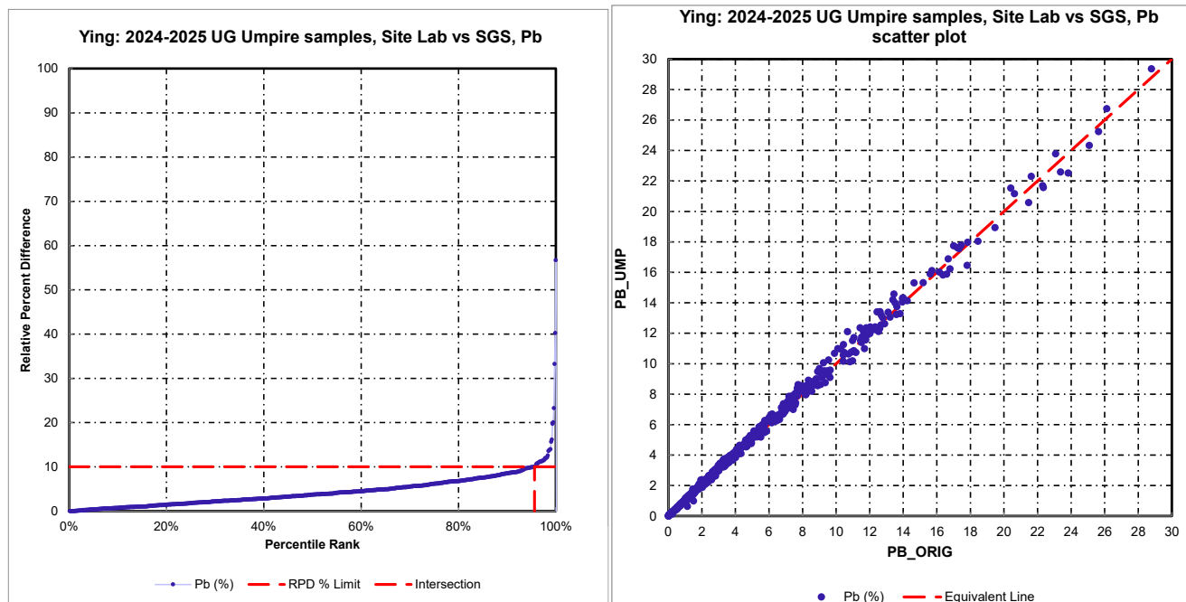
Figure 11.18 Ying umpire RPD and scatter plots of Pb (UG samples, Site Lab, SGS Umpire Lab)
