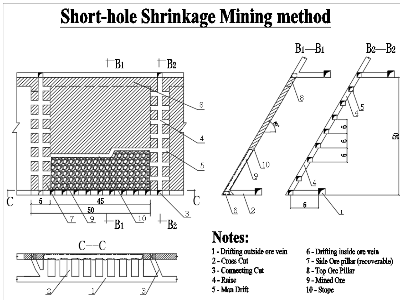
Figure 16.6 Shrinkage stoping method
